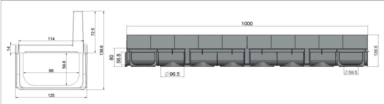
Technical sections of Plastic drain channel with plastic slotted grating
