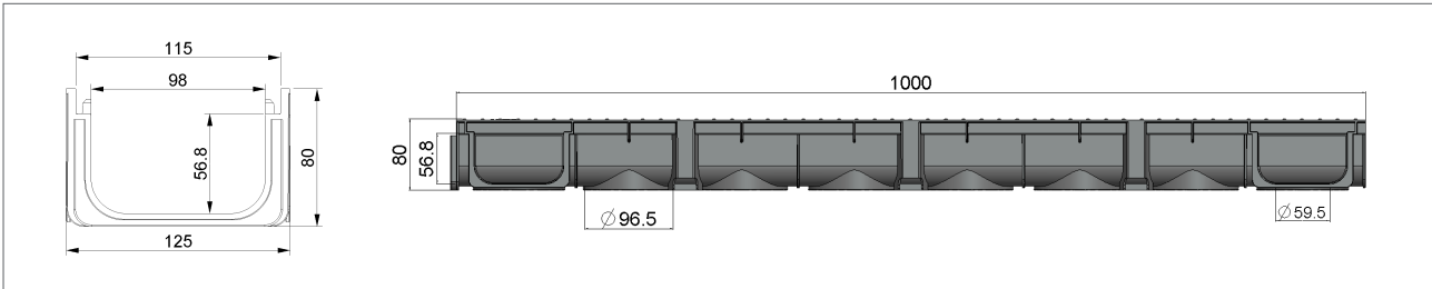
Technical sections of Plastic drain channel
